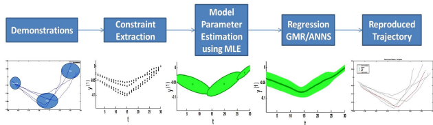
Figure 1: Block diagram explaining the individual steps of the algorithm.
